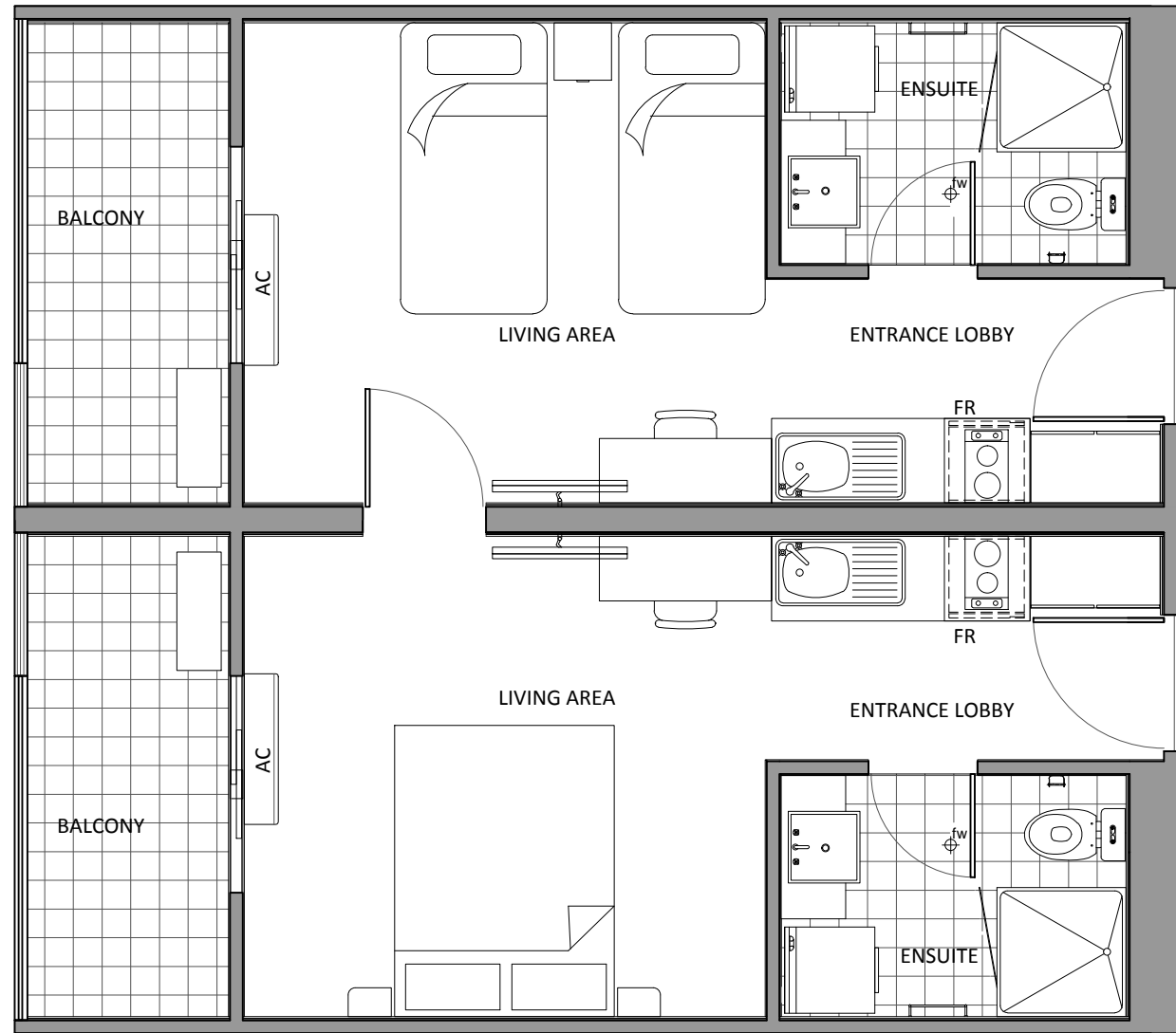
FAMILY ROOM PLAN
