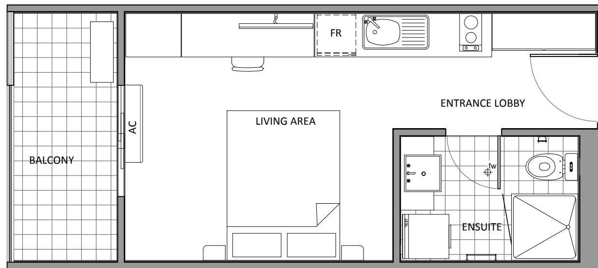
SINGLE ROOM PLAN
